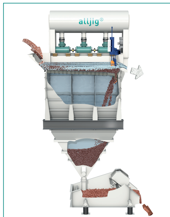
Vibrating feeder discharge
