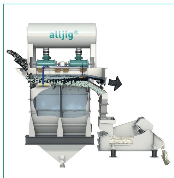
alljig® - GR grain size max. 100 mm (4")
